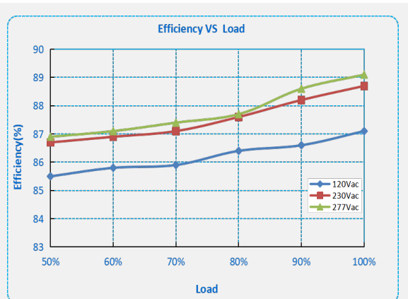
L1-100X-036/048/054
